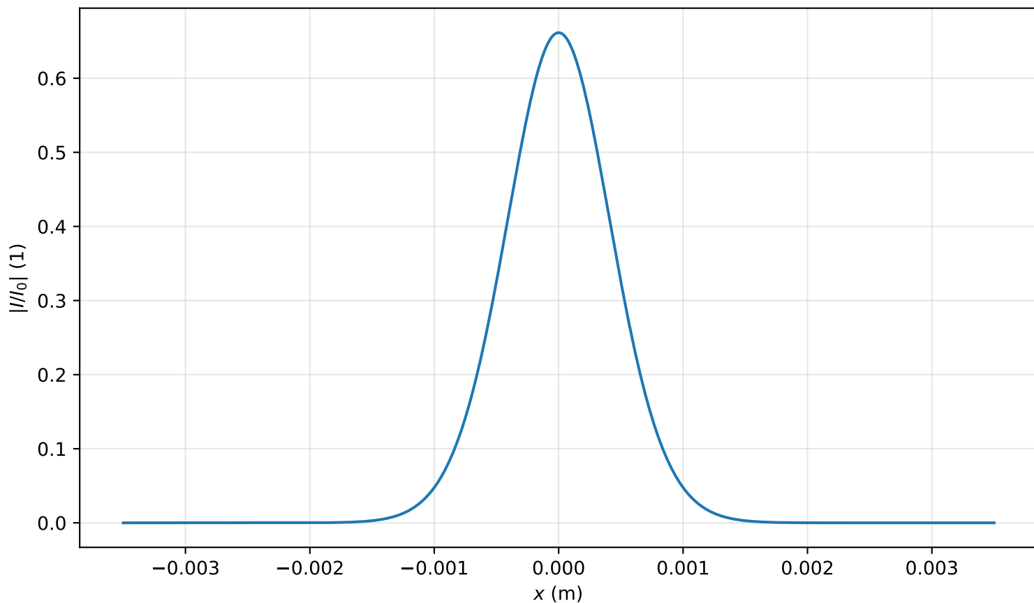
Intensity profile I(x, y = 0, z = 1.751m)/I_0 , P_{in}=0.2P_{cr} , artificial time
